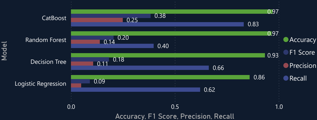
High Accuracy Alone Is Misleading — F1 Score Decides the Winner
