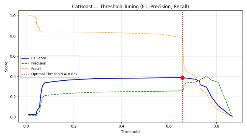
Threshold Tuning Chart
