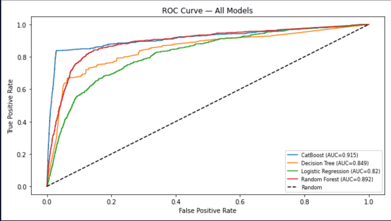
ROC Curve — All Models
