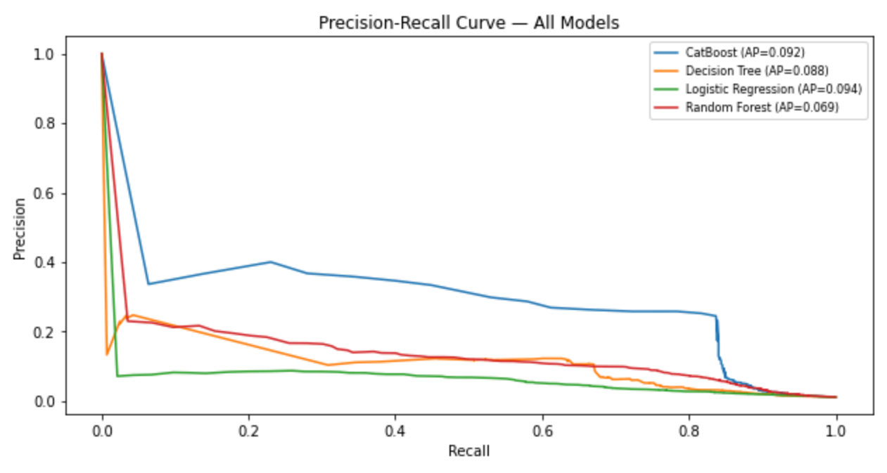
Precision-Recall Curve — All Models
